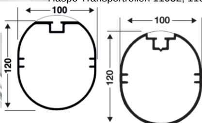
Haspo Transportrollen 11032, 11033, 11035, 11036
