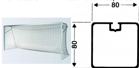
Kleinfeldtor 3 x 2m in Bodenhülsen Haspo 150
