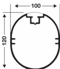
Haspo Transportrollen 11032, 11033, 11035, 11036
