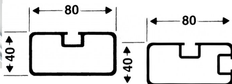
Haspo Transportrollen 11032, 11033, 11035, 11036
