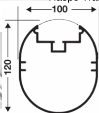
Haspo Transportrollen 11032, 11033, 11035, 11036
